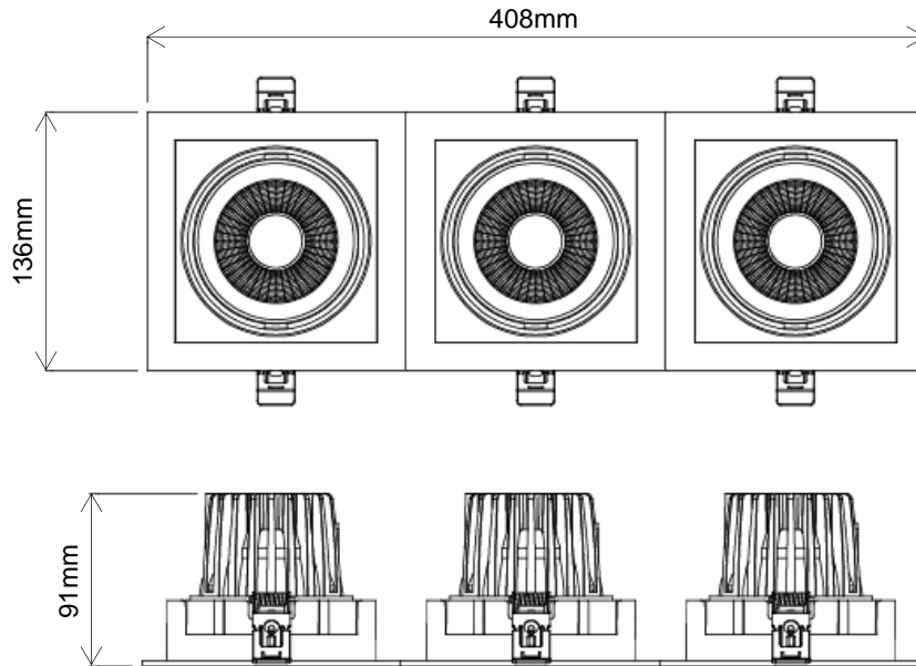
Cut-out Ø390mm - Ø120mm
